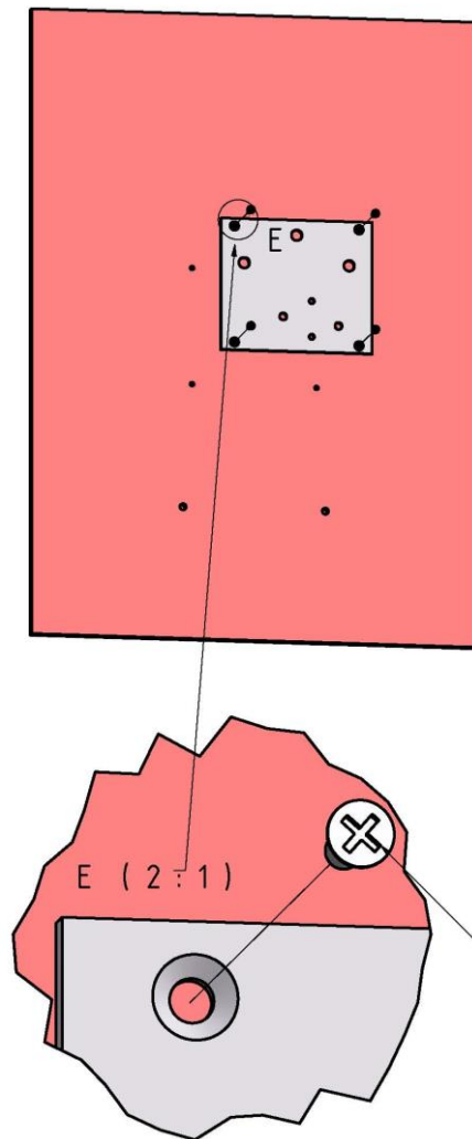
Stap 1: montage extra koellichaam
