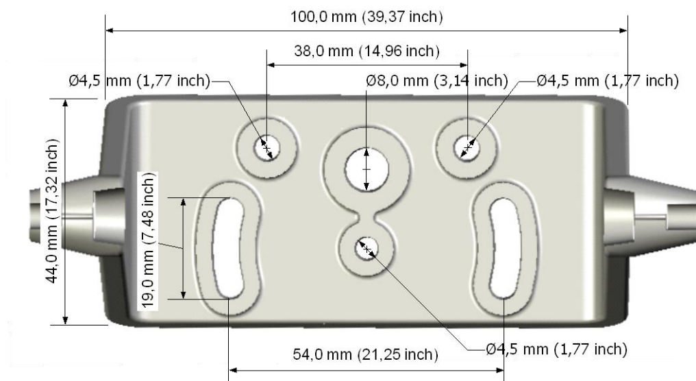
Fig. 1: Retaining bracket
