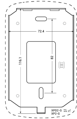
Drilling Template
